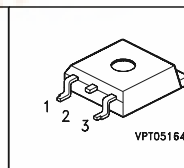
P-TO263-3-2
