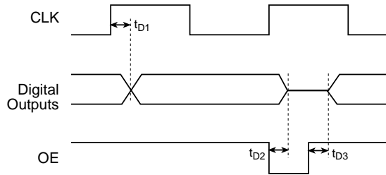
Figure 5 – Timing Diagram 2
