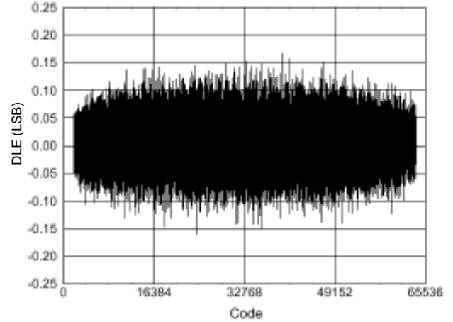
Typical Differential Linearity Error (DLE)
