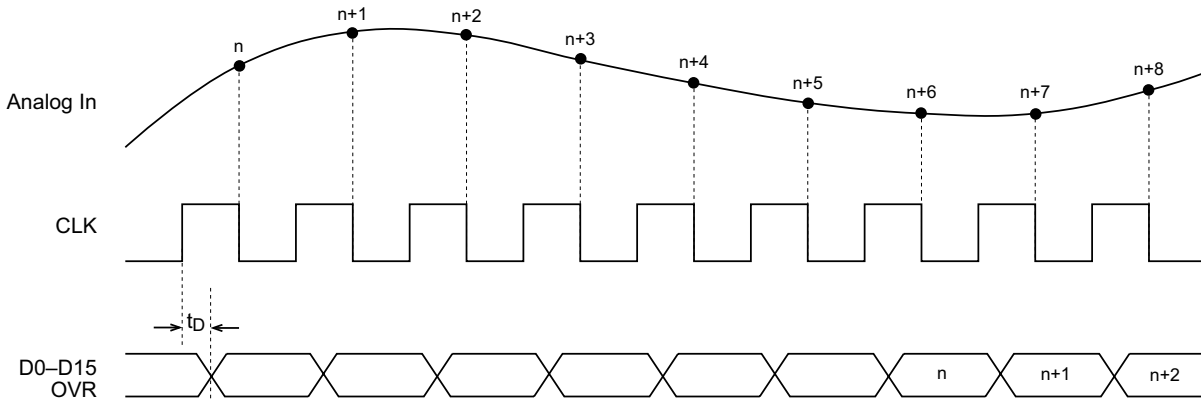
Figure 3 – Timing Diagram 1
