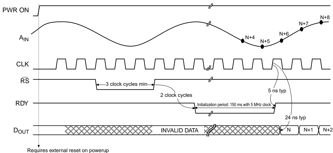
Figure 1 – Device Initialization Timing
