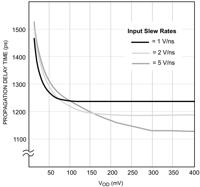
PROPAGATION DELAY vs INPUT OVERDRIVE VOLTAGE
