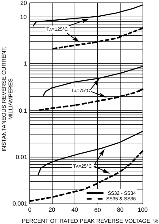
FIG. 4 - TYPICAL REVERSE CURRENT CHARACTERISTICS
