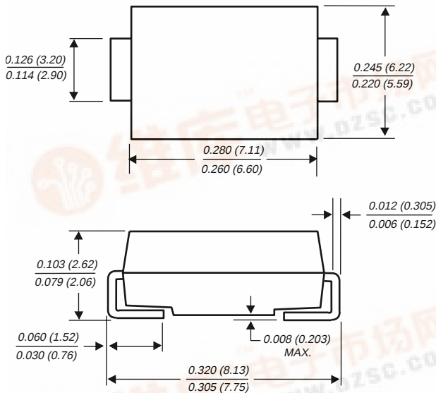
DO-214AB
