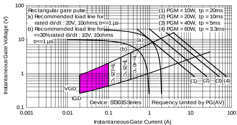
Fig. 15 - Gate Characteristics
