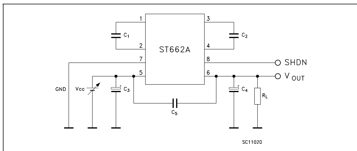
Figure 9 : Test Circuit
