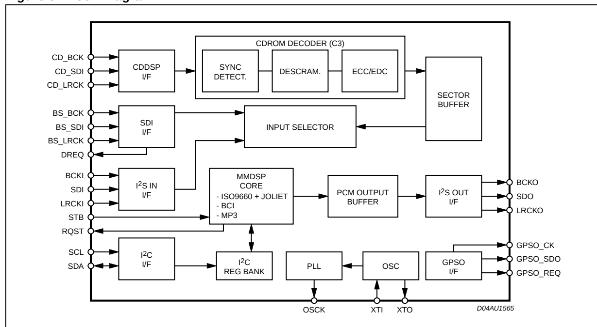
Figure 3. Block Diagram
