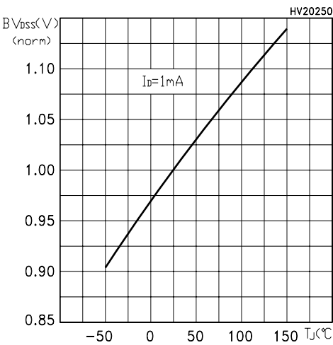
Figure 17: Normalized BV_{DSS} vs Temperature
