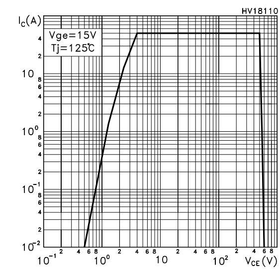
Turn-Off SOA
