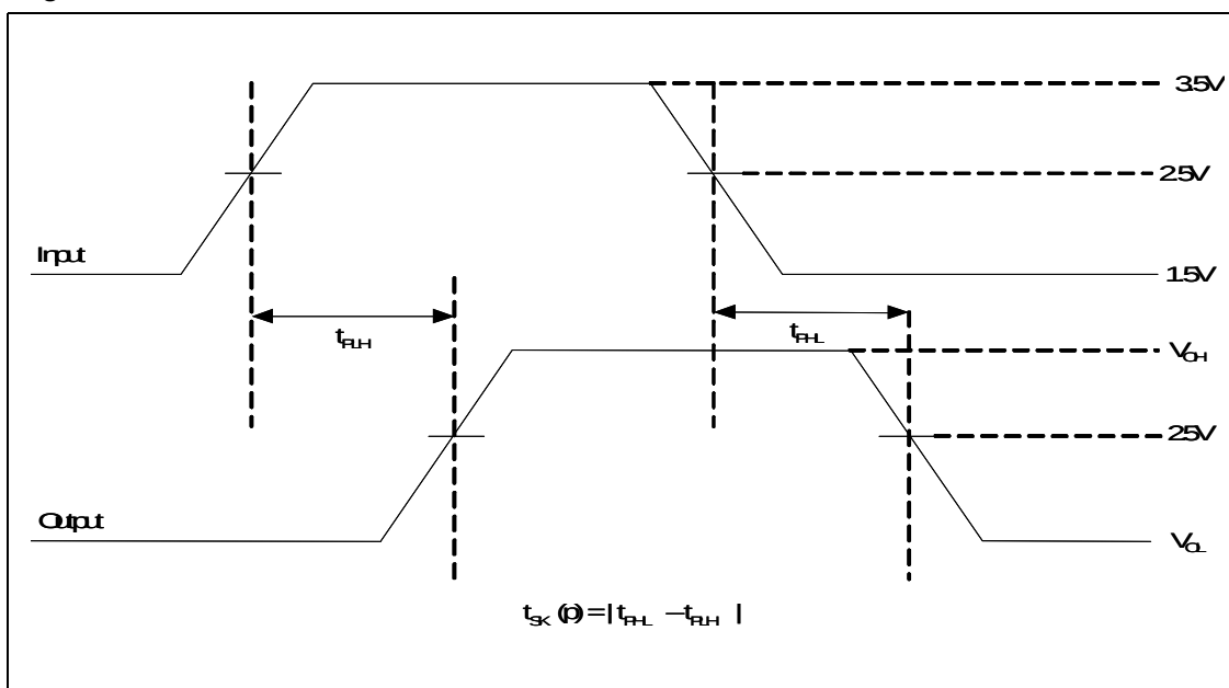
Figure 7. Pulse skew
