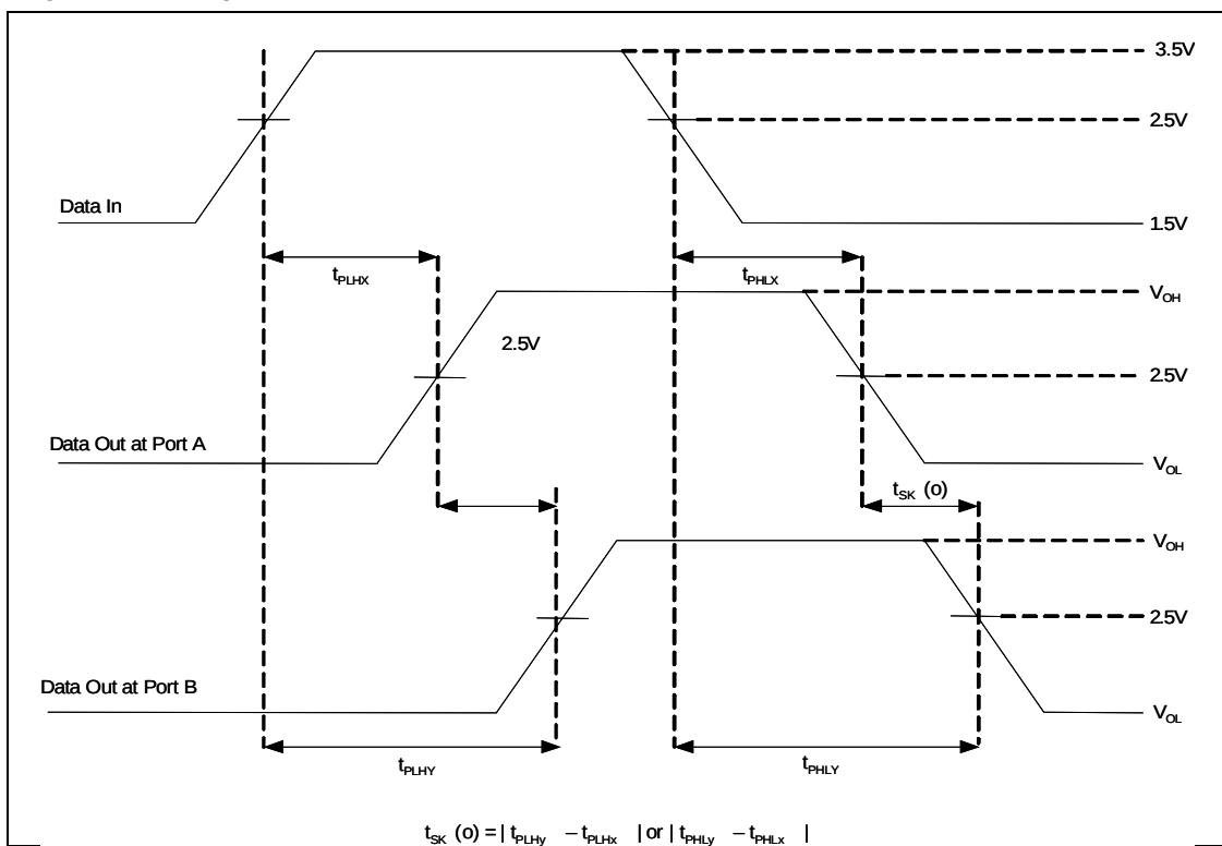
Figure 5. Output skew
