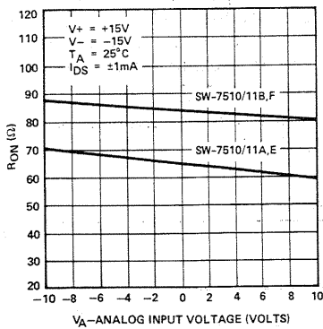
"ON" RESISTANCE ( R_{ON} ) vs ANALOG VOLTAGE ( V_A )
