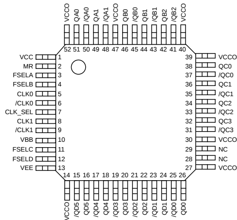
52-Pin LQFP (LQFP-52)
