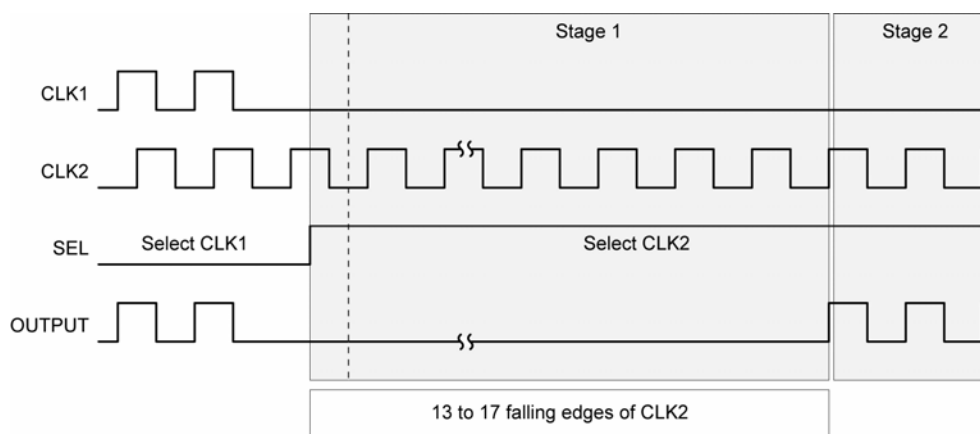
Timing Diagram 3
