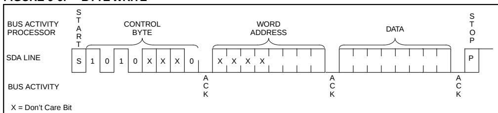
FIGURE 6-6: BYTE WRITE
