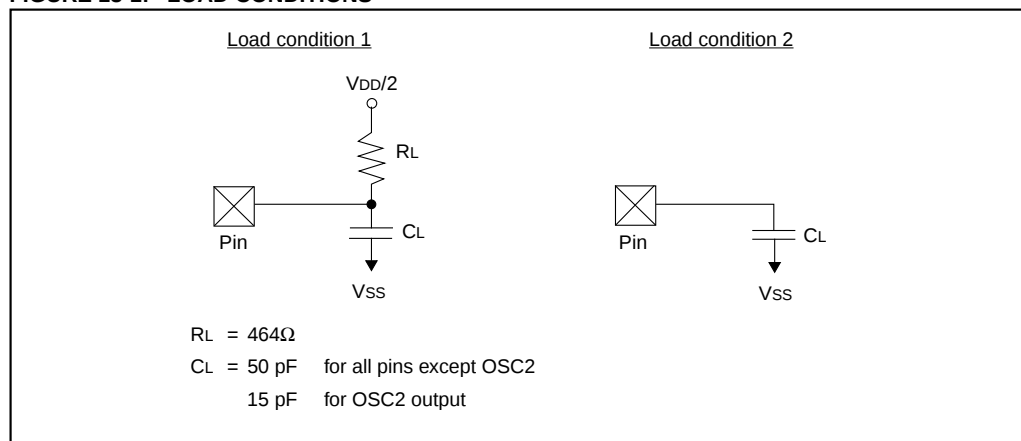
FIGURE 13-1: LOAD CONDITIONS
