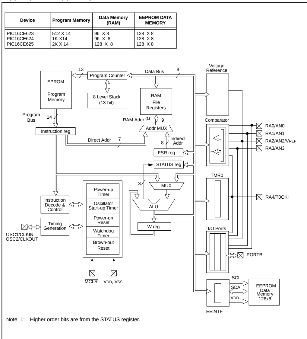
FIGURE 3-1: BLOCK DIAGRAM
