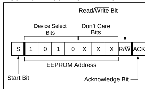
FIGURE 6-4: CONTROL BYTE FORMAT
