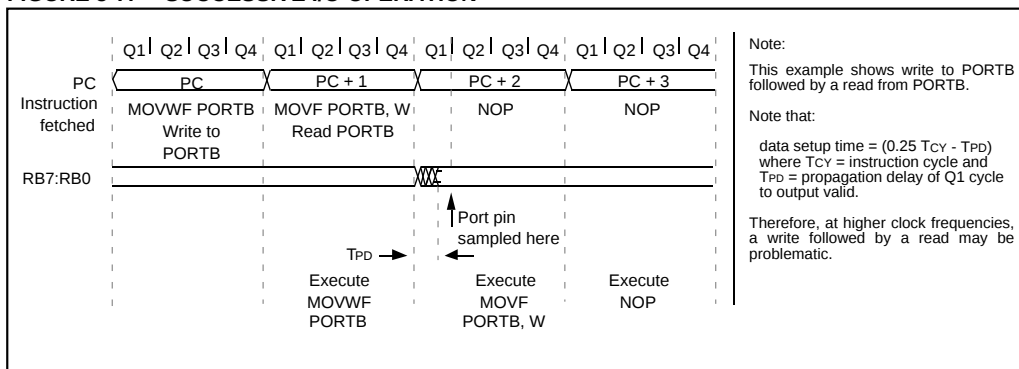
FIGURE 5-7: SUCCESSIVE I/O OPERATION
