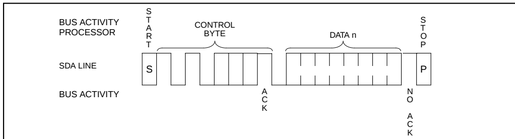
FIGURE 6-9: RANDOM READ
