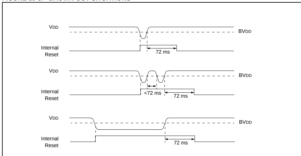
FIGURE 10-8: BROWN-OUT SITUATIONS
