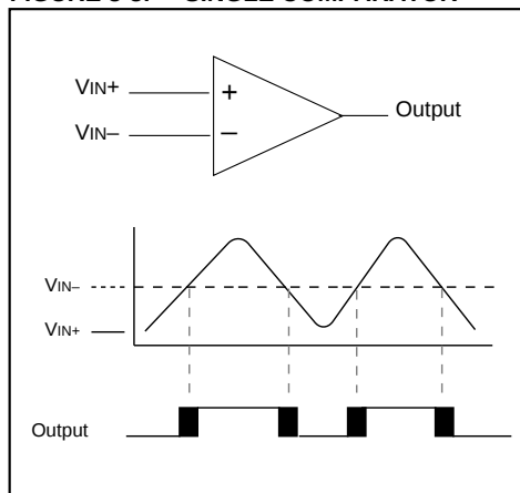
FIGURE 8-3: SINGLE COMPARATOR
