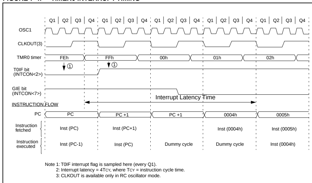
FIGURE 7-4: TIMER0 INTERRUPT TIMING
