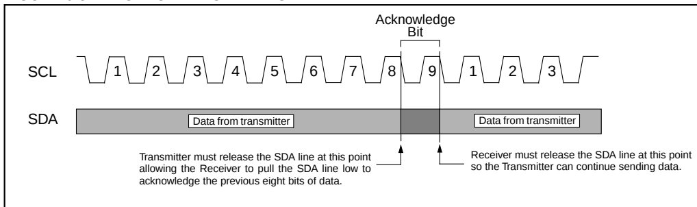
FIGURE 6-3: ACKNOWLEDGE TIMING
