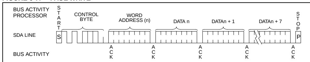
FIGURE 6-7: PAGE WRITE
