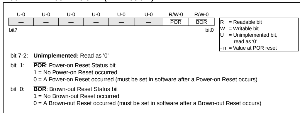
FIGURE 4-11: PCON REGISTER (ADDRESS 8Eh)
