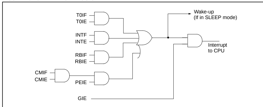
FIGURE 10-15: INTERRUPT LOGIC
