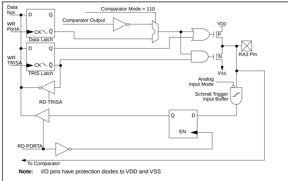
FIGURE 5-3: BLOCK DIAGRAM OF RA3 PIN
