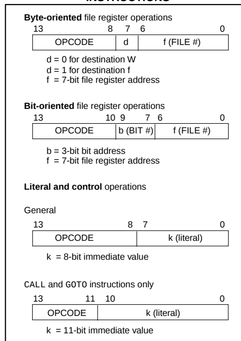
FIGURE 11-1: GENERAL FORMAT FOR INSTRUCTIONS
