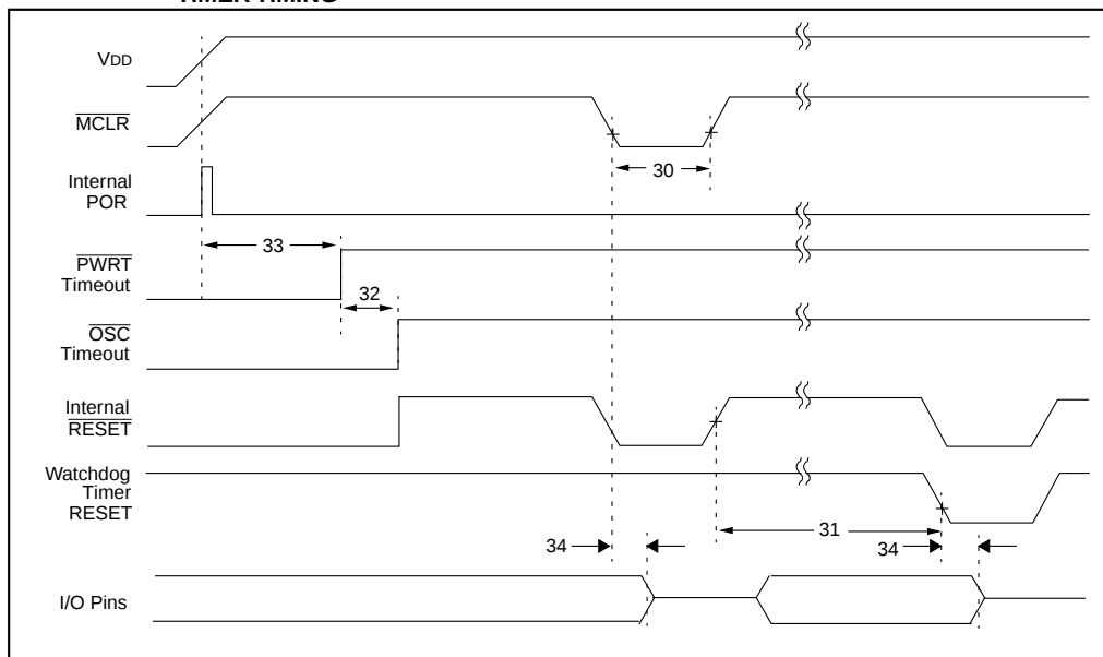
FIGURE 13-5: BROWN-OUT RESET TIMING
