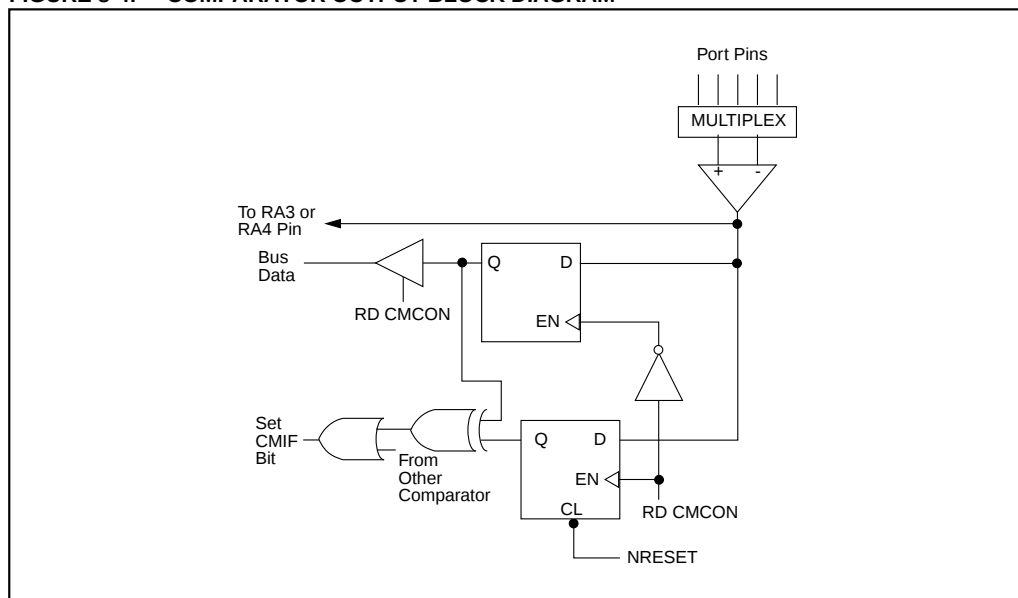
FIGURE 8-4: COMPARATOR OUTPUT BLOCK DIAGRAM
