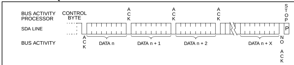
FIGURE 6-10: SEQUENTIAL READ
