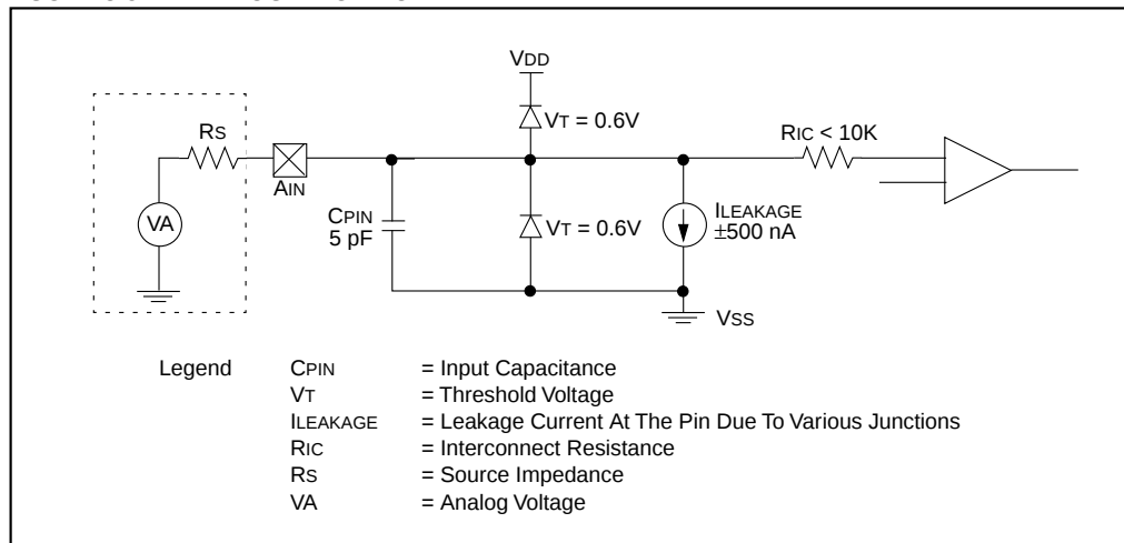
FIGURE 8-5: ANALOG INPUT MODEL
