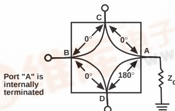
Figure 1. 2 Way, In-Phase (0°) Power Divider/Summer, or ISO-T
