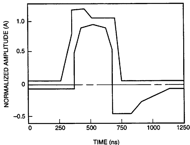
T1 Isolated-Pulse Corner Points According to FCC Part 68
