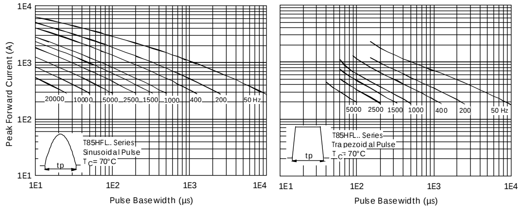
Fig. 43 - Frequency Characteristics
