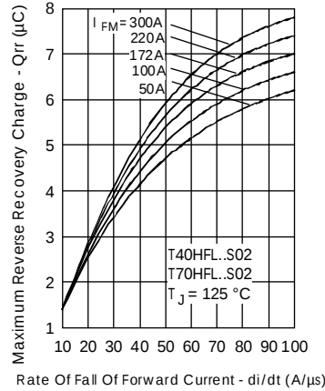
Fig. 20 - Recovery Charge Characteristics
