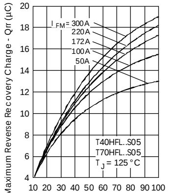
Fig. 23 - Recovery Charge Characteristics
