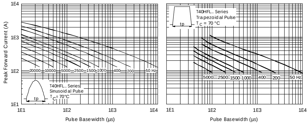
Fig. 37 - Frequency Characteristics
