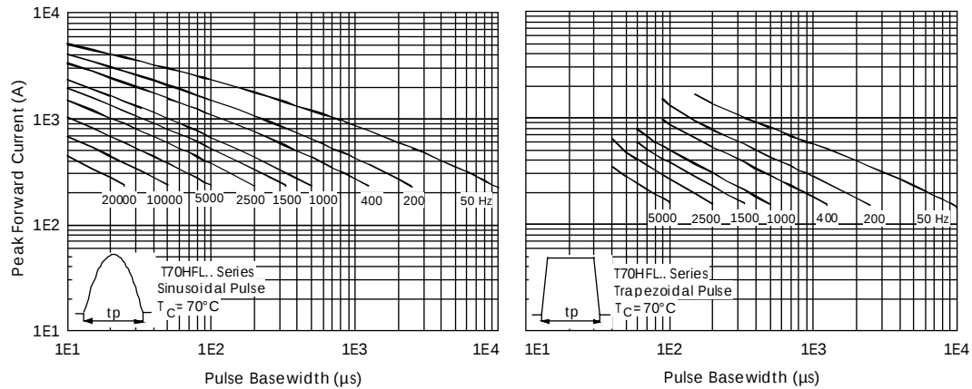
Fig. 40 - Frequency Characteristics
