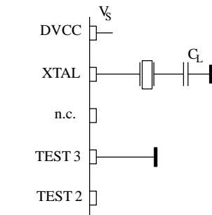
Figure 4. XTO peripherals
