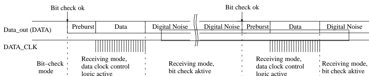
Figure 26. Output of digital noise at the end of the data stream
