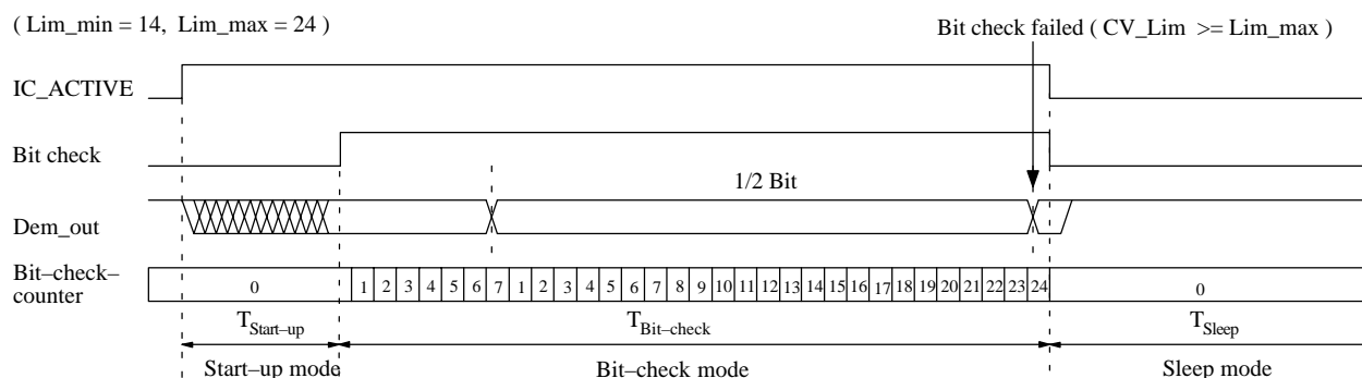
Figure 13. Timing diagram for failed bit check (condition: CV_Lim >= Lim_max)
