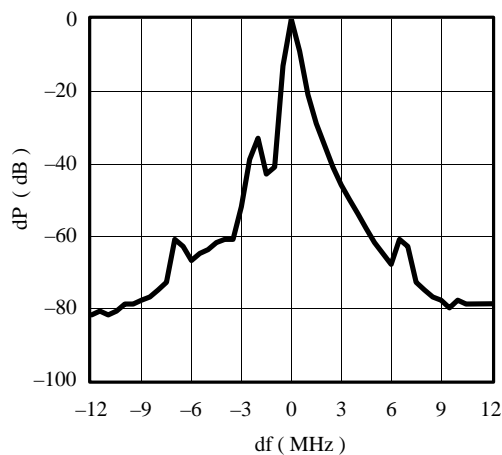
Figure 7. Wide band receiving frequency response
