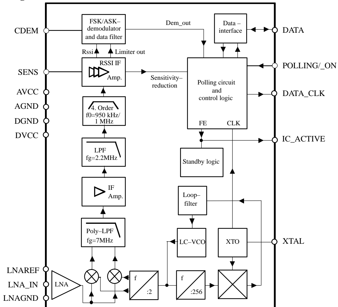
Figure 3. Block diagram
