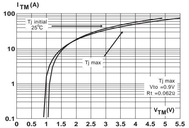
Fig.8 : On-state characteristics (maximum values).
