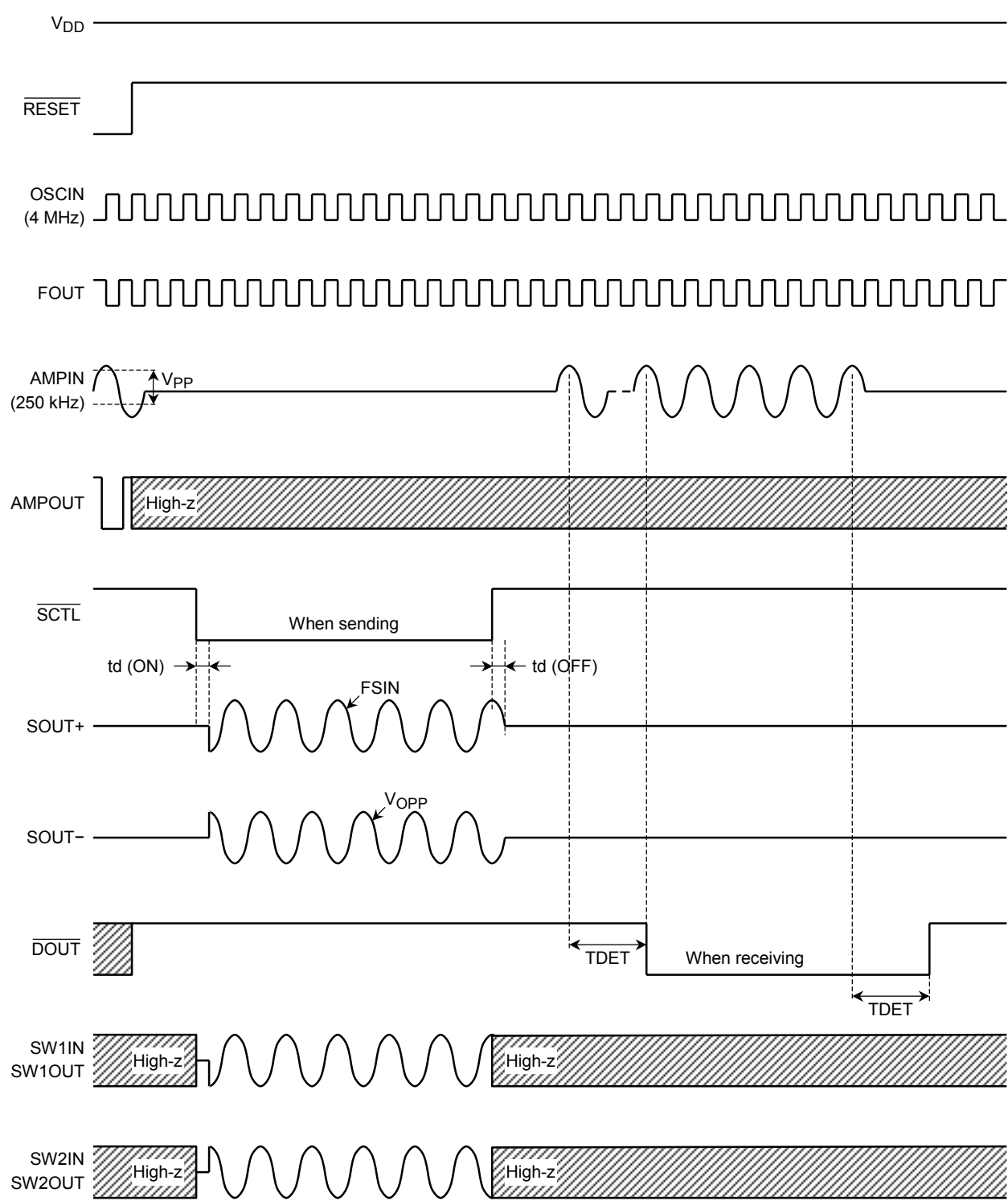
Timing Chart (SOUT+ = SW1IN, SW1OUT, SOUT- = SW2IN, SW2OUT)
