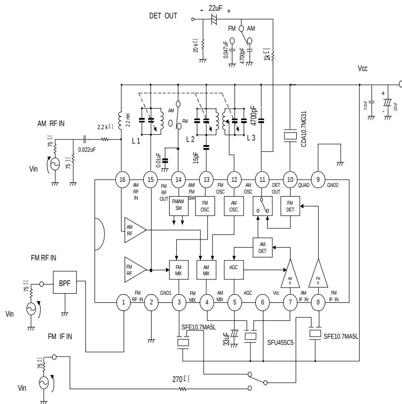
TEST CIRCUIT 1
