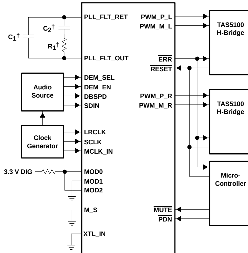
Figure 5–1. Connection Diagram, Slave Mode (typical)
