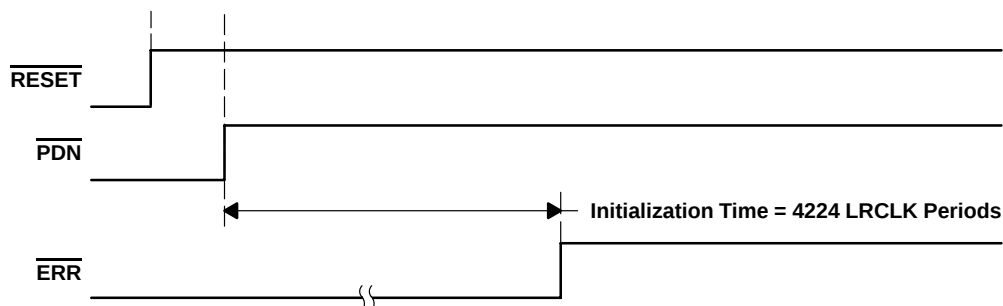
Figure 2–1. Power-Up Timing (RESET preceding PDN)
