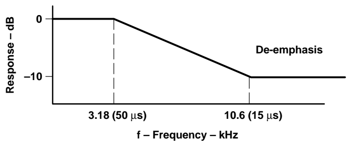
Figure 6. De-Emphasis Filter Characteristics
