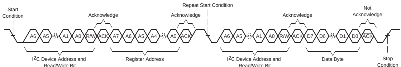
Figure 2-16. Single-Byte Read
