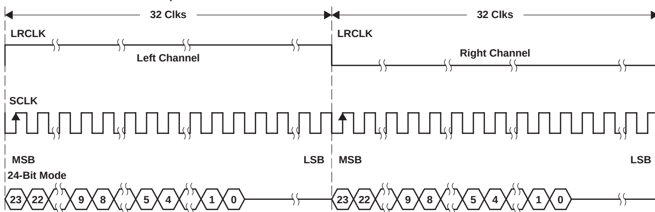
2-Channel Left-Justified Stereo Input
