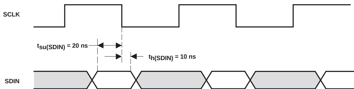
Figure 5-11. DSP Absolute Timing
