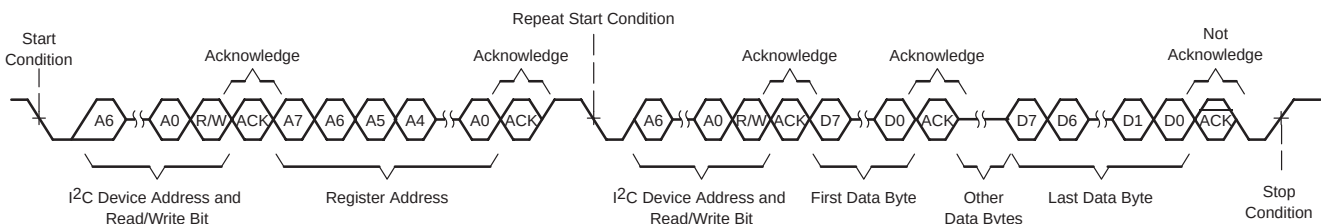
Figure 2-17. Multiple-Byte Read
