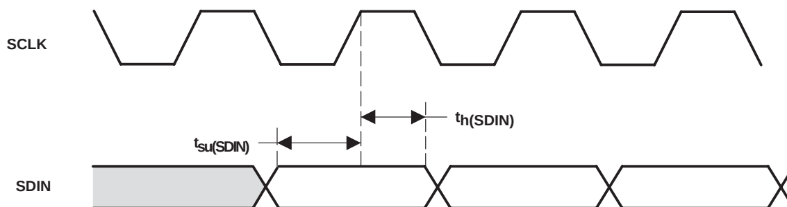
Figure 5–6. Right-Justified, I²S, Left-Justified Serial-Protocol Timing
