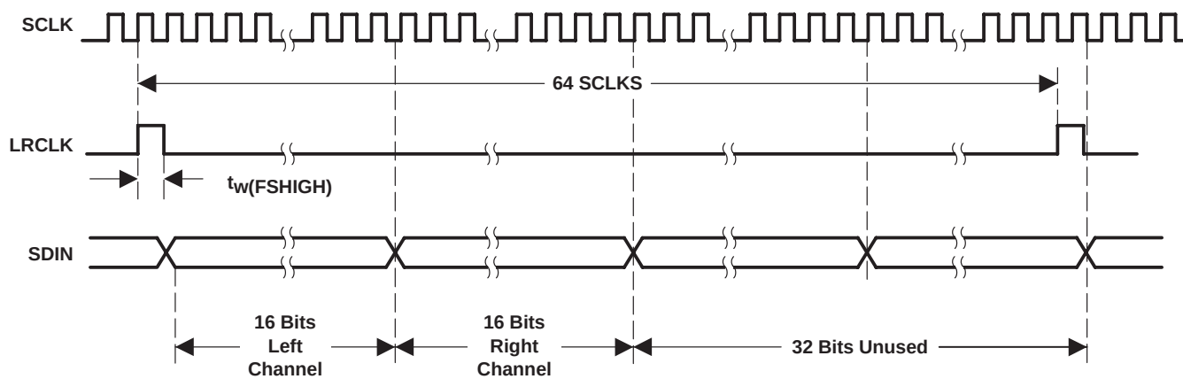
Figure 5-10. DSP Serial-Port Expanded Timing
