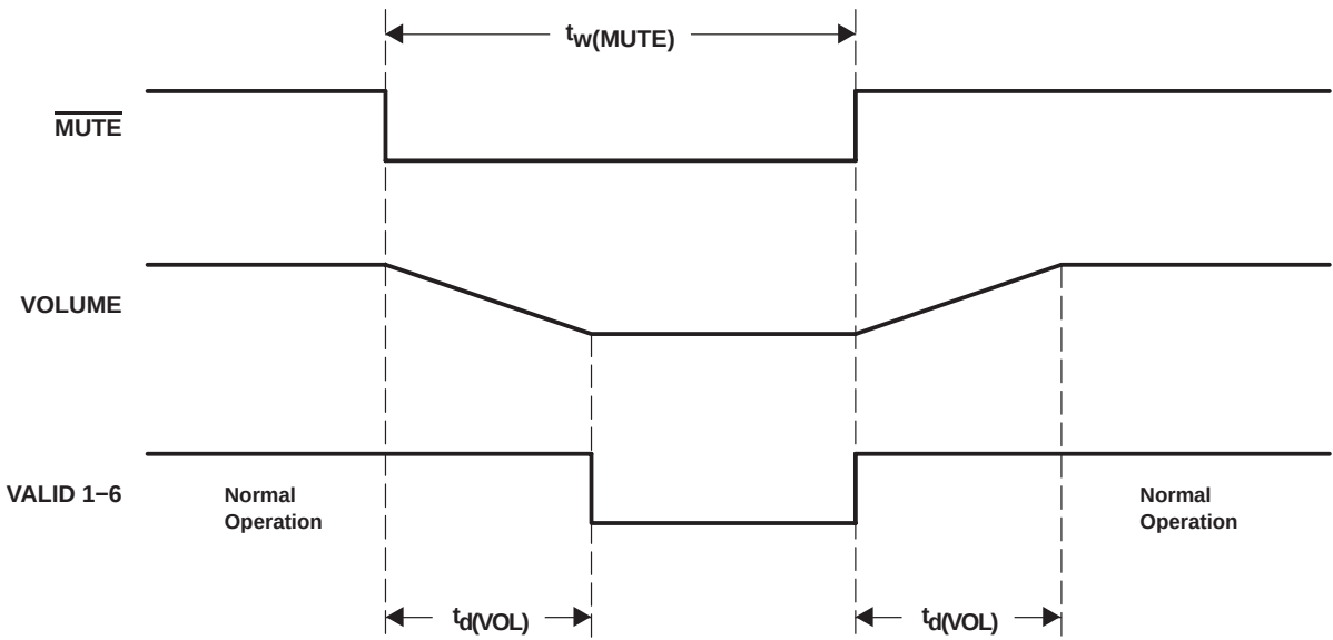
Figure 5-5. Mute Timing
