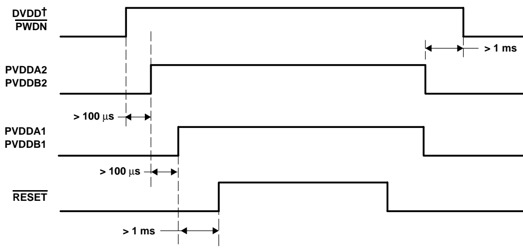
Figure 3. Power-Up/Power-Down Sequence
