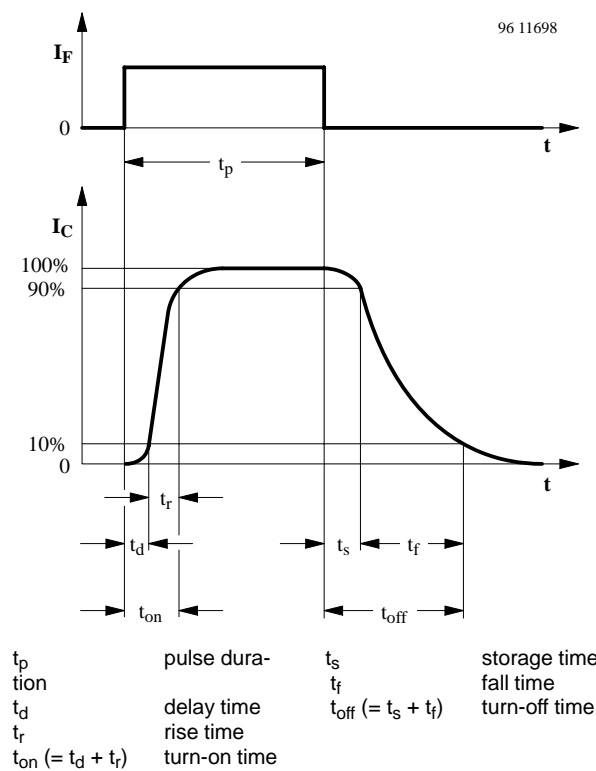
Figure 4. Switching times
