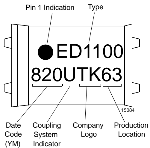
Figure 12. Marking example
