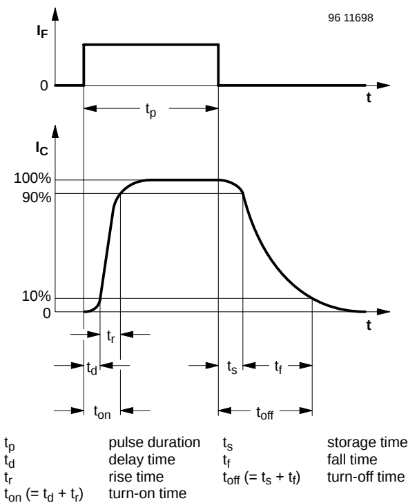
Figure 5. Switching times
