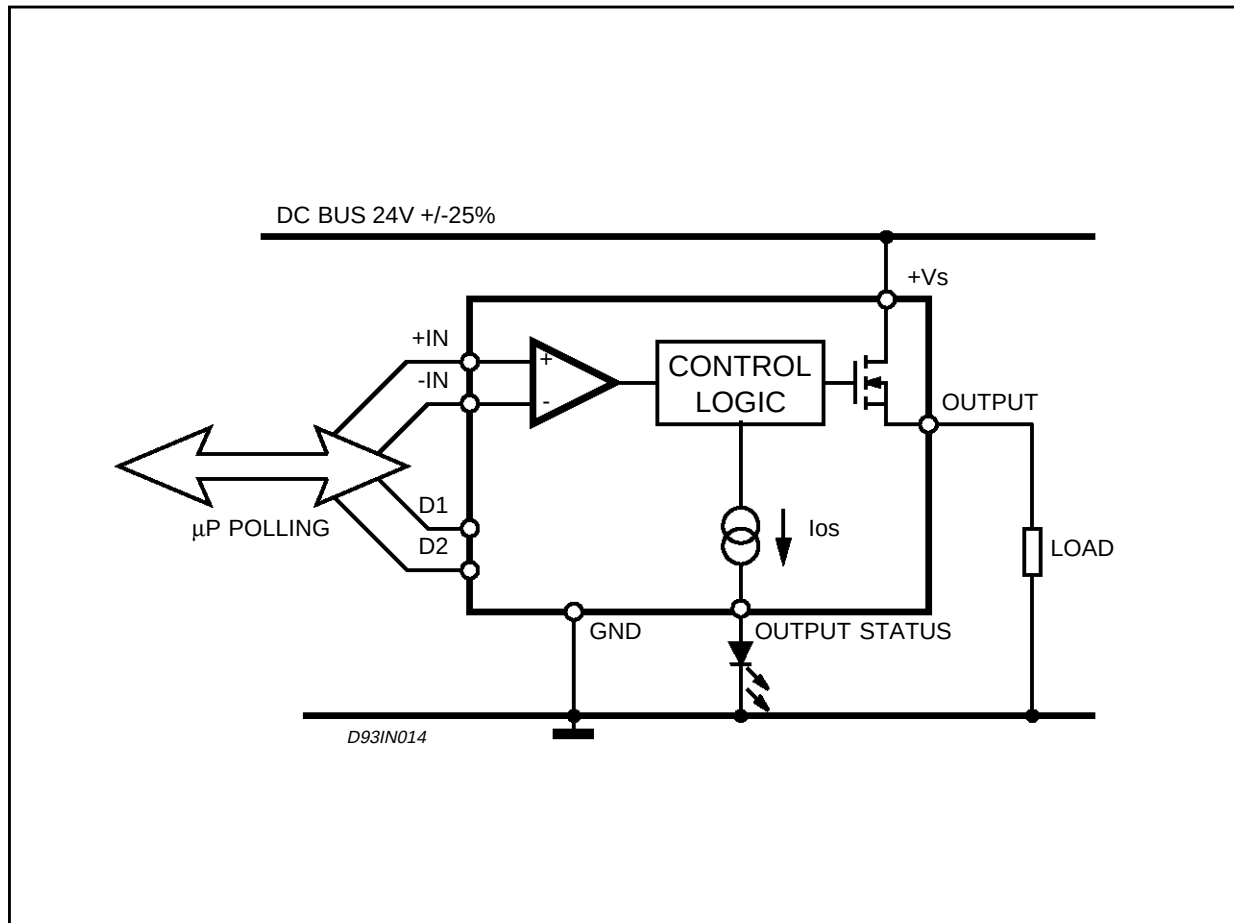
Figure 5: Application Circuit.
