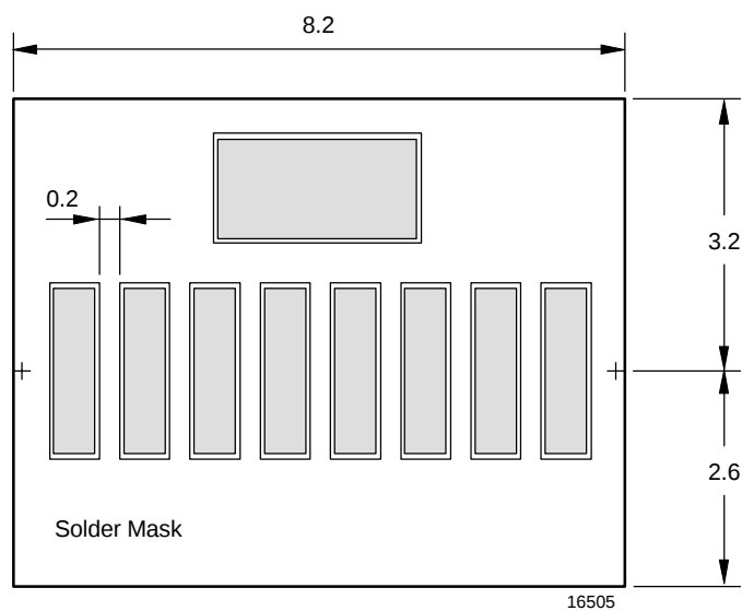
Figure 7. Adjacent Land Keep-out and Solder Mask Areas
