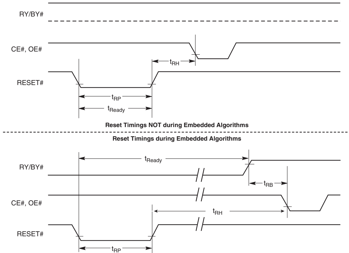
Figure I5. RESET# Timings
