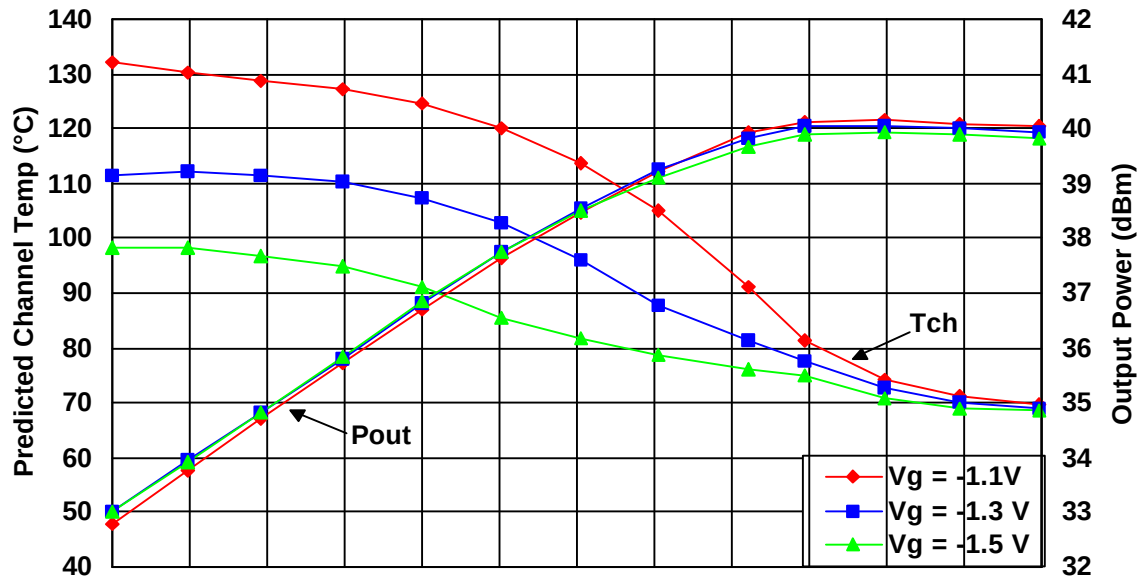
TGF4124-EPU RF Performance for V_d = 7.0 V, F = 2.3 GHz, and T_A = 25^\circ\text{C} Quiescent I_d is 2.24 A ( V_g = -1.1 V), 1.81 A ( V_g = -1.3 V), and 1.37 A ( V_g = -1.5 V)
