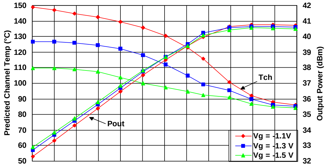
TGF4124-EPU RF Performance for V_d = 8.0 V, F = 2.3 GHz, and T_A = 25^\circ\text{C} Quiescent I_d is 2.17 A ( V_g = -1.1 V), 1.80 A ( V_g = -1.3 V), and 1.40 A ( V_g = -1.5 V)
