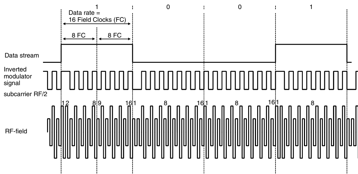
Figure 18. Example of PSK Encoding with Data Rate RF/16
