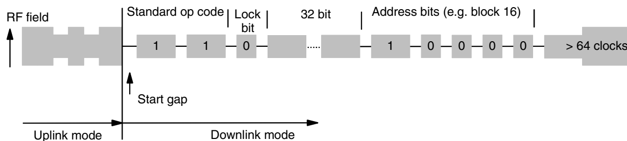
Figure 8. Downlink Protocol
