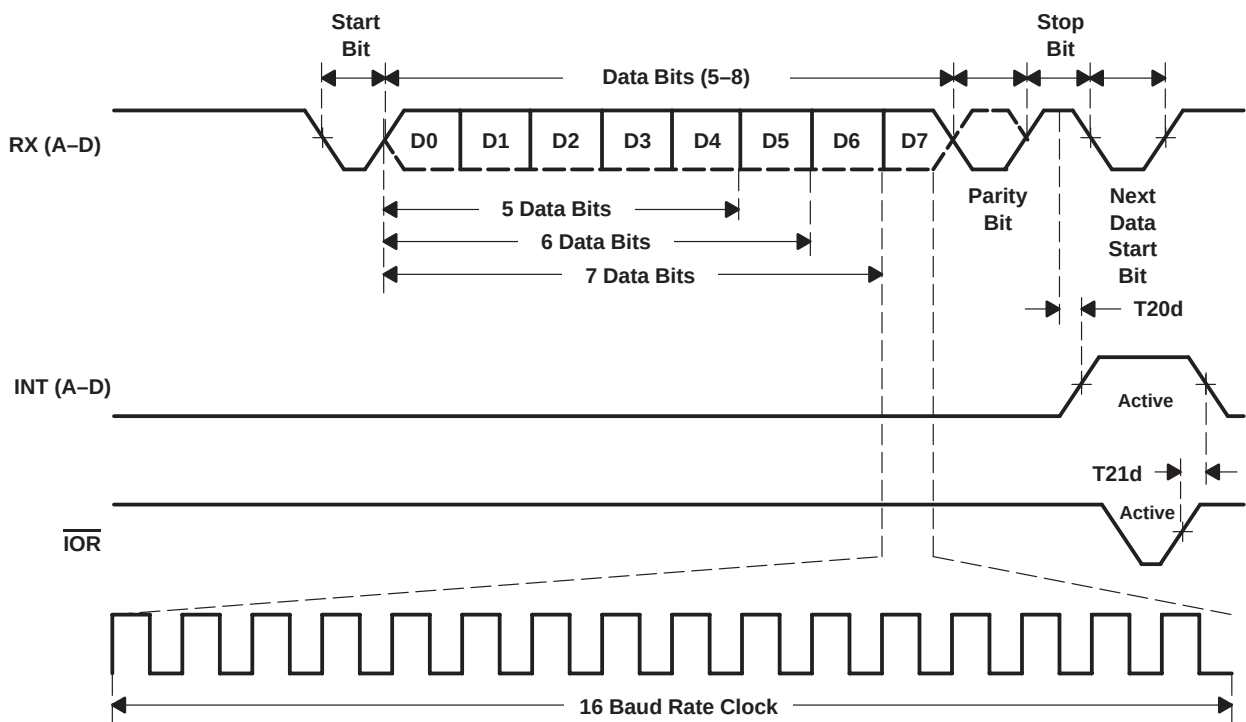
Figure 15. Receive Timing
