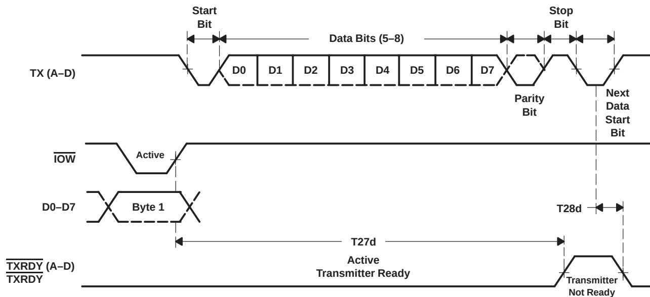
Figure 19. Transmit Ready Timing in None FIFO Mode
