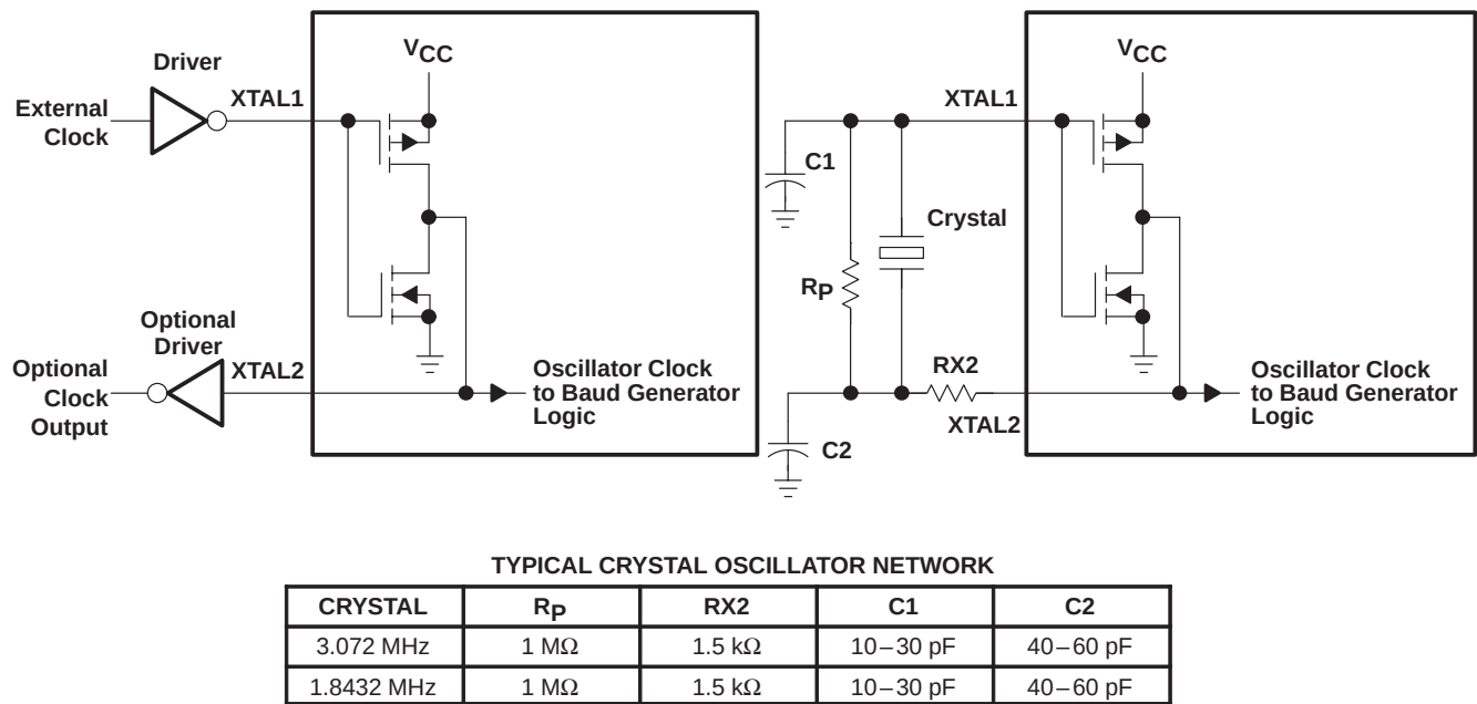
Figure 10. Typical Crystal Clock Circuits †
