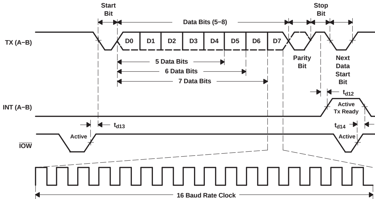
Figure 18. Transmit Timing
