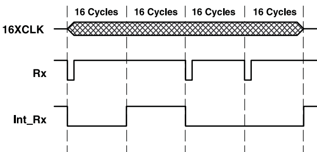
Figure 31. IrDA-SIR Decoding Scheme – Macro View
