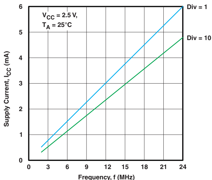
Figure 12. Supply Current vs Frequency ( V_{CC} = 2.5\text{ V} )
