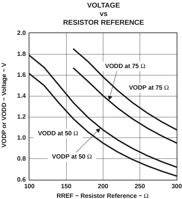
Figure 14. Differential Transmitter Voltage
