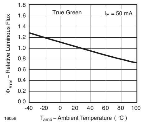
Figure 24. Rel. Luminous Flux vs. Ambient Temperature
