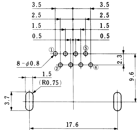
PCB mounting hole layout (Connector mounting side)
