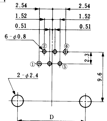
PCB mounting hole layout (Connector mounting side)
