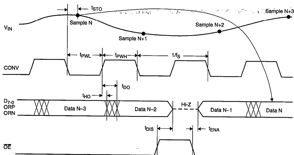
Figure 2. Conversion Timing
