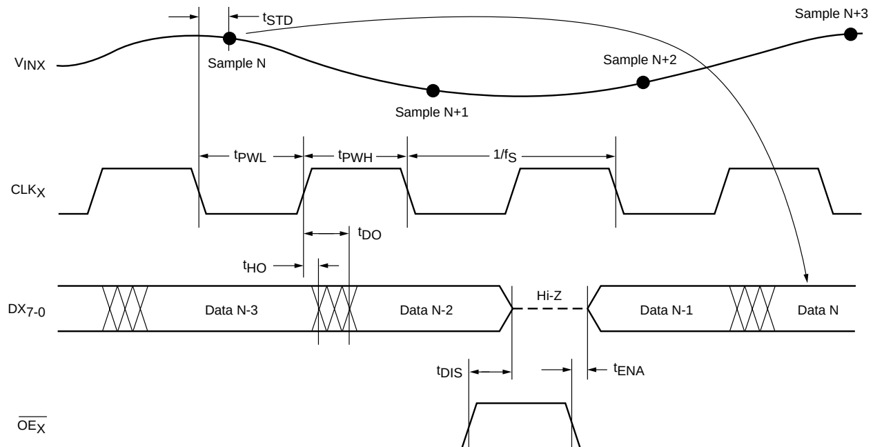
Figure 1. Timing
