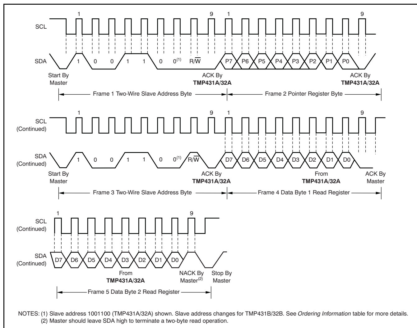
Figure 19. Two-Wire Timing Diagram for Two-Byte Read Format
