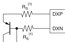
(b) Diode-Connected Transistor
