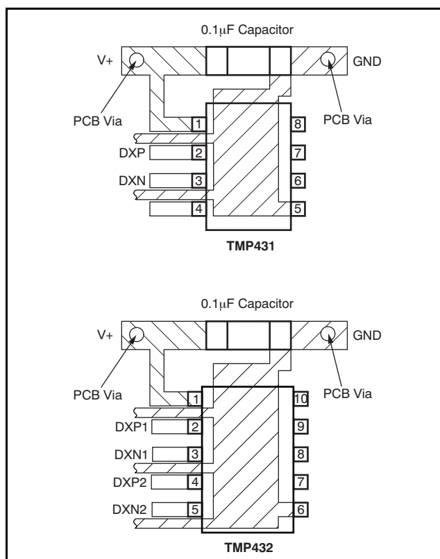
Figure 23. Suggested Bypass Capacitor Placement
