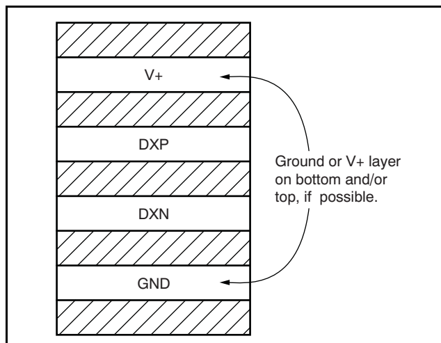
Figure 22. Example Signal Traces
