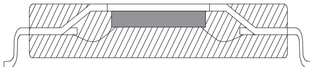
Figure 10. Leadframe Downset
