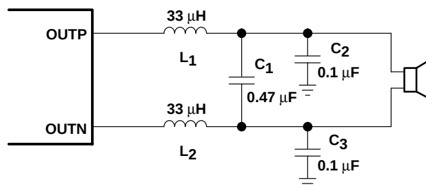
Figure 40. Typical LC Output Filter, Cutoff Frequency of 41 kHz, Speaker Impedance = 8 Ω
