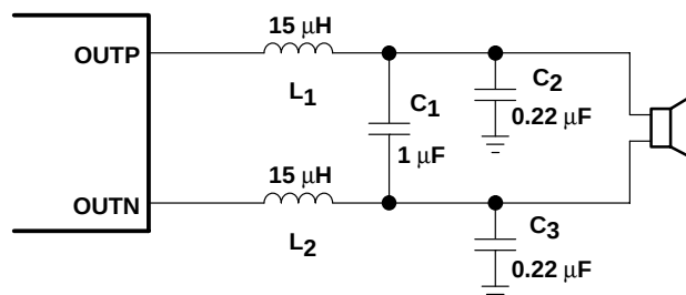
Figure 39. Typical LC Output Filter, Cutoff Frequency of 41 kHz, Speaker Impedance = 4 Ω
