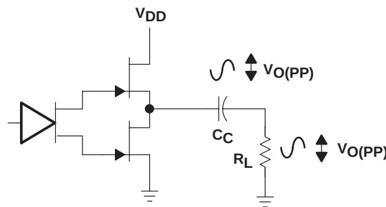
Figure 35. Single-Ended Configuration
