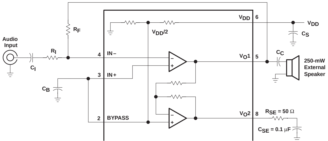
Figure 38. Singled-Ended Mode
