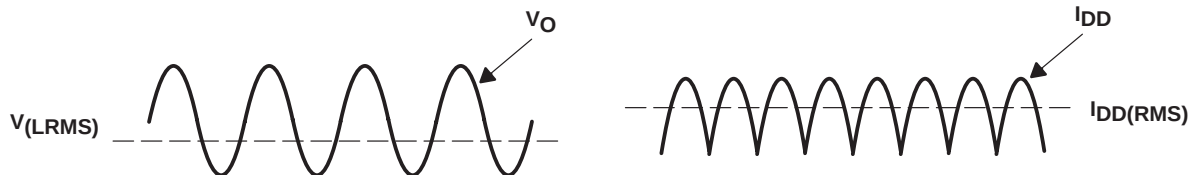
Figure 36. Voltage and Current Waveforms for BTL Amplifiers
