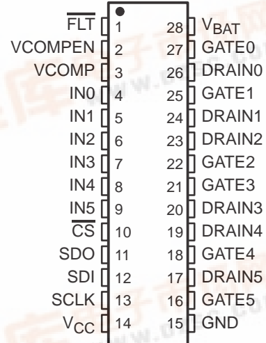
DB PACKAGE (TOP VIEW)
