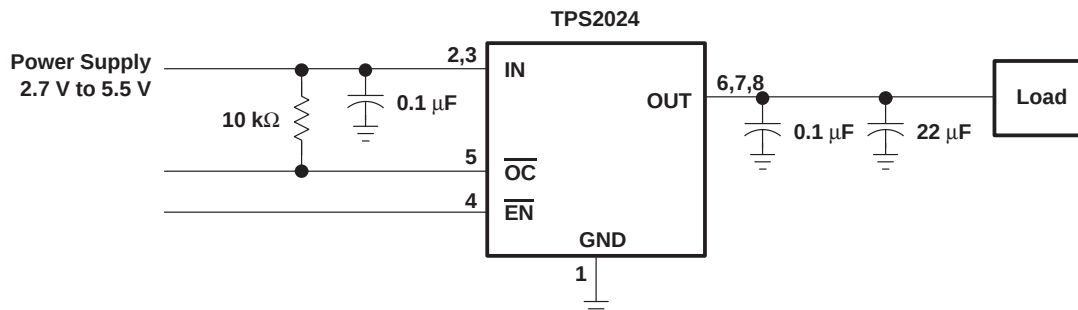
Figure 38. Typical Application
