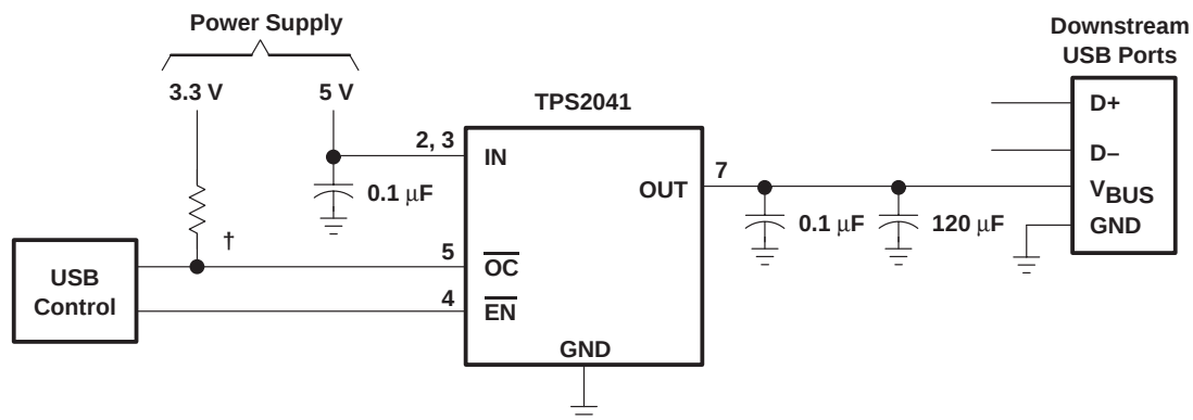
Figure 31. One-Port Solution
