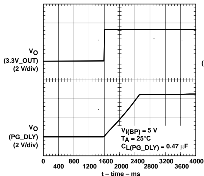
Figure 9. PG_DLY Rise Time With a 0.47- \mu\text{F} Capacitor
