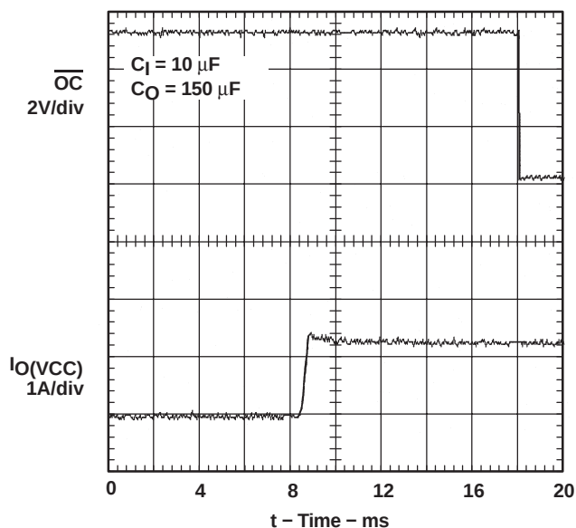
Figure 5. \overline{\text{OC}} Response With 5VIN-to-xVCC Switch Output Turned on Into a Short
