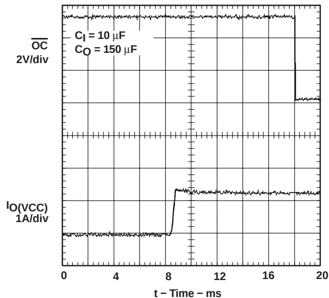
Figure 6. \overline{\text{OC}} Response With 3.3VIN-to-xVCC Switch Output Turned on Into a Short
